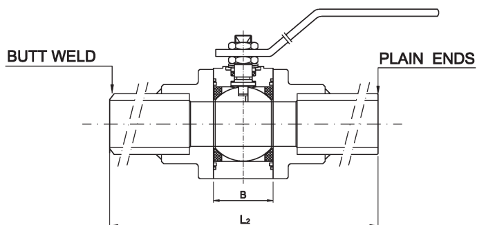
WELDED NIPPLES
